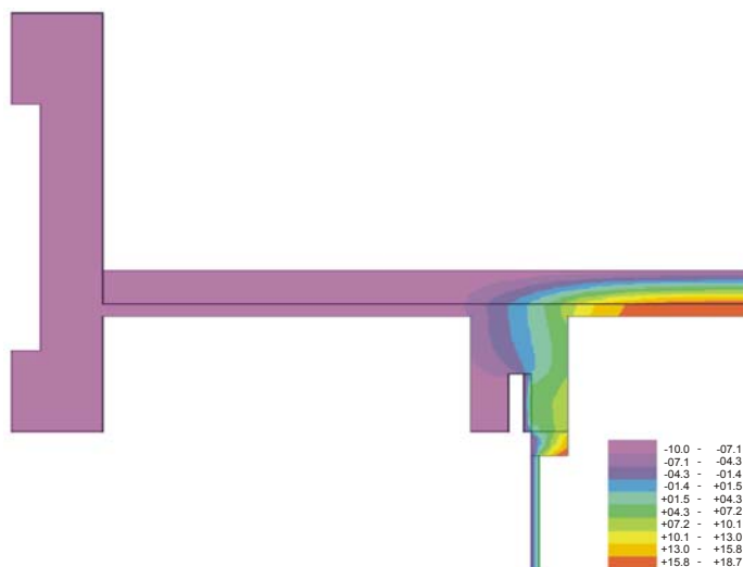
Figure 3: Typical thermal bridge of a projecting roof with an concrete attic
