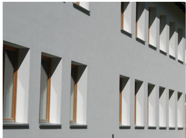
Figure 26: Windows mounted centred within reveal (Source: Obereder Hans, A+ ZT GmbH)
