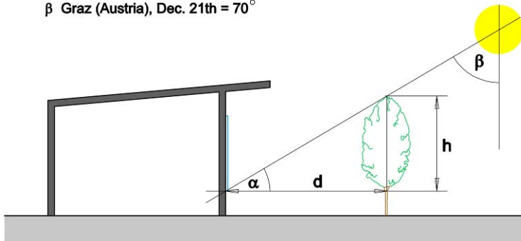
Figure 35: Shadow casted by a tree upon a south-oriented façade (Source: Colourface [18])
