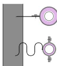
Figure 21: Fixing pipes to avoid sound transmission
