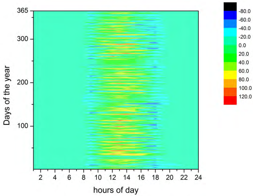
Figure 68. Coloured contour graph of net exported energy. Units are in kW. Case study MB4
