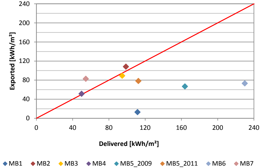
Figure 13. ZEB status exported v. delivered for the monitored buildings. Figures are in kW·h/m² (Primary Energy)
