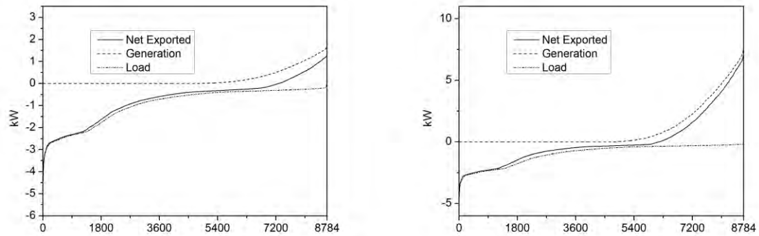
Figure 51. Duration curve for generation, load and net exported electricity. Case studies MB1 (left) and MB2 (right).
