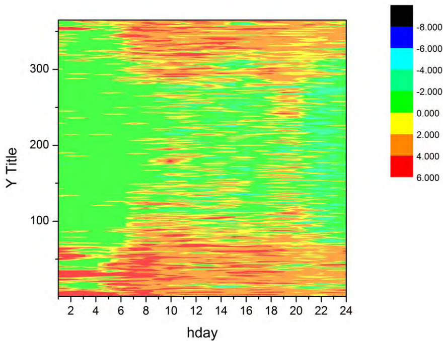
Figure 69. Coloured contour graph of net exported energy. Units are in kW. Case study MB6
