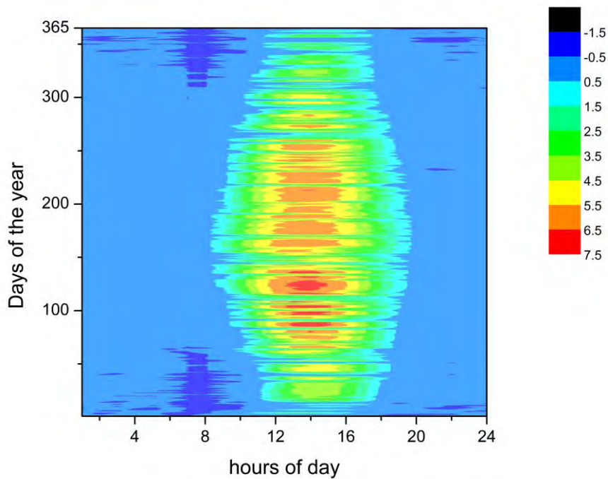
Figure 71. Coloured contour graph of net exported energy. Units are in kW. Case study SB4
