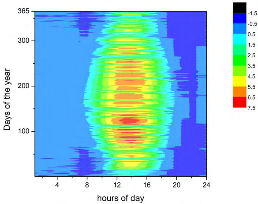
Figure 70. Coloured contour graph of net exported energy. Units are in kW. Case study SB3
